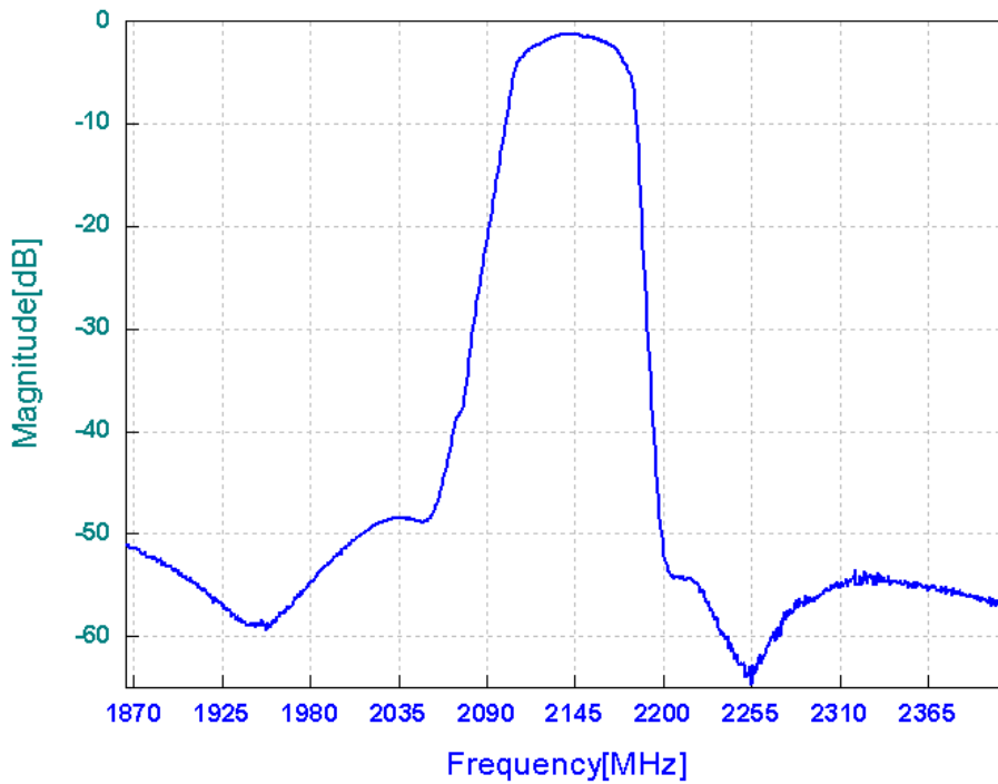
Frequency Response
